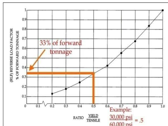
Fig 6- determine the reverse load
