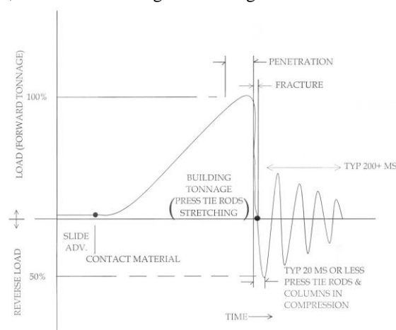
Fig 1 - Break through shock
