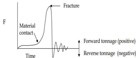
Fig 3-blanking cycle without shock
