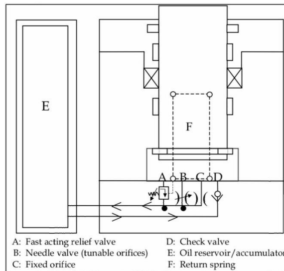
Fig 4-Construction of hydraulic damper
